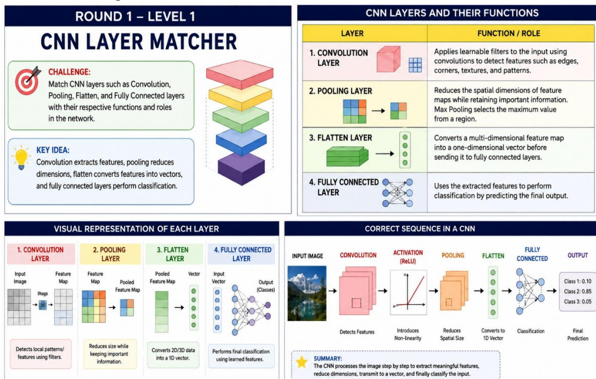
Figure 1: CNN Layer Matcher – Visual Representation of CNN Layers and Their Functions
