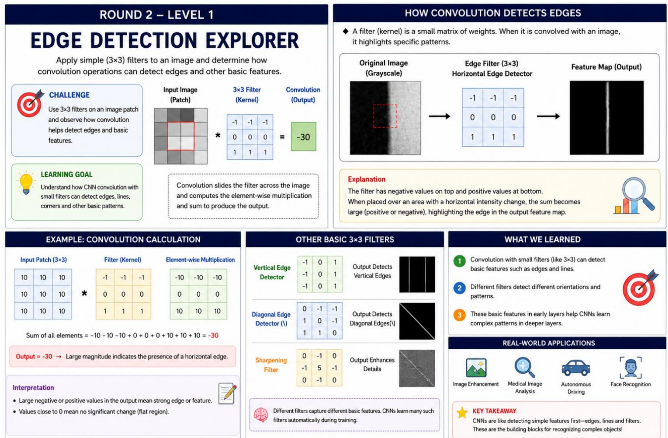
Figure 2: Edge Detection Explorer
